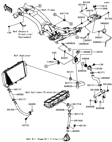
D-3 Water Pipe
